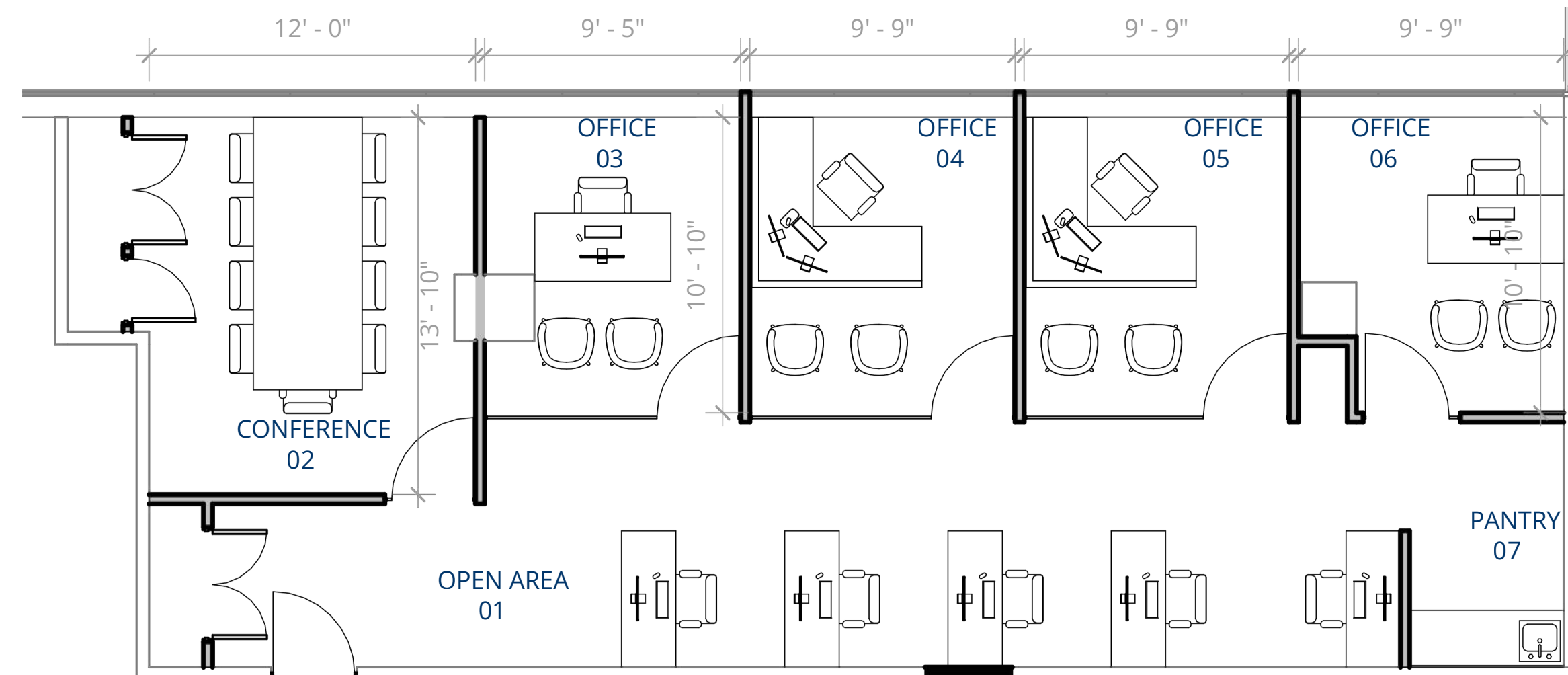
Proposed Plan
